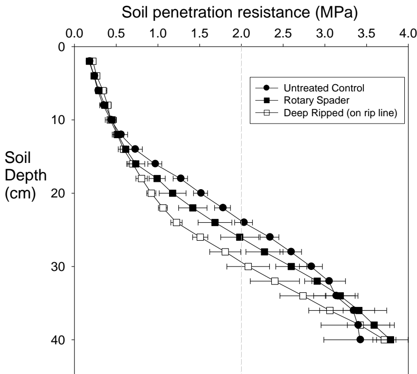
Figure 1: Impact of rotary spading and deep ripping on soil penetration resistance measured using a cone penetrometer in megapascals (MPa) in a yellow deep sand at Marchagee when the soil was wet. Note that at 2MPa or more crop root growth rates are reduced.
